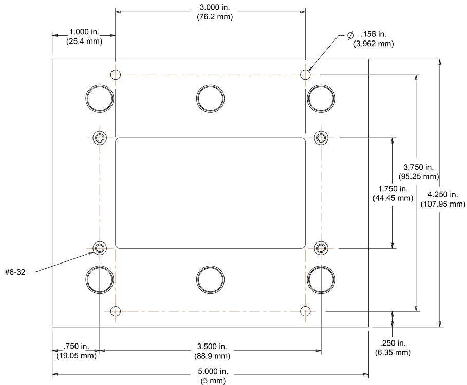
Figure 4: 8010-130 Customizable Test Board dimensions
