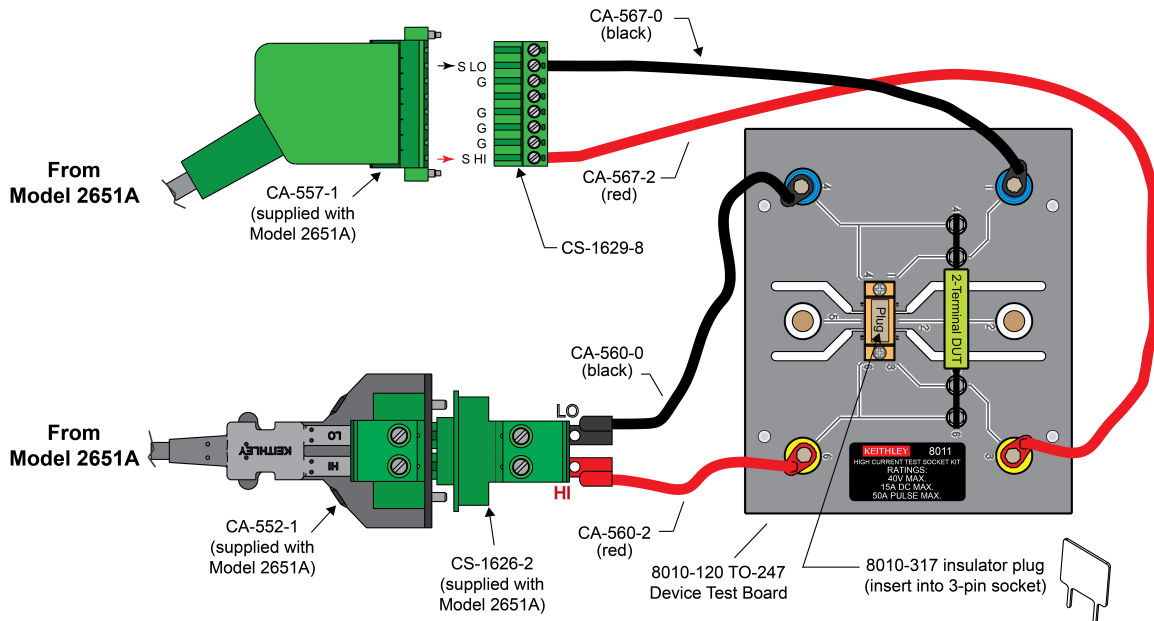
Figure 6: Connections for two-terminal device test (remote sense)
