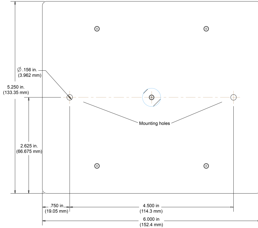
Figure 3: Mounting plate dimensions
