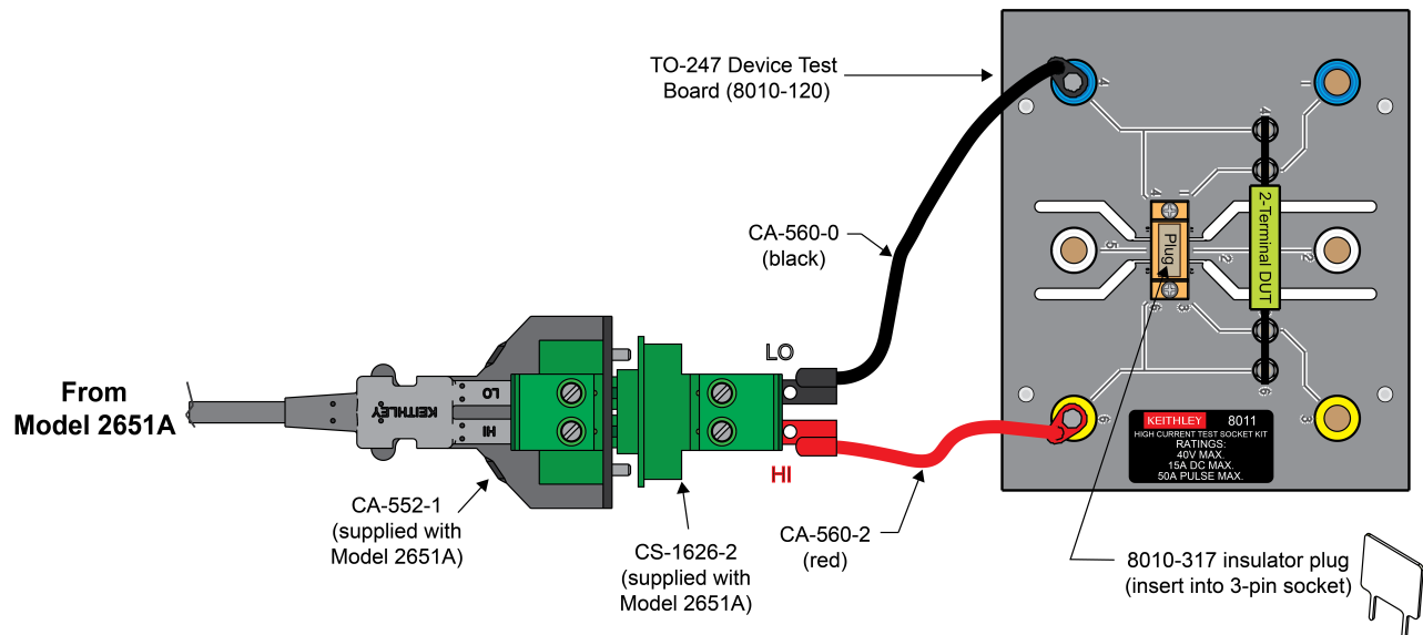
Figure 5: Connections for two-terminal device test (local sense)
