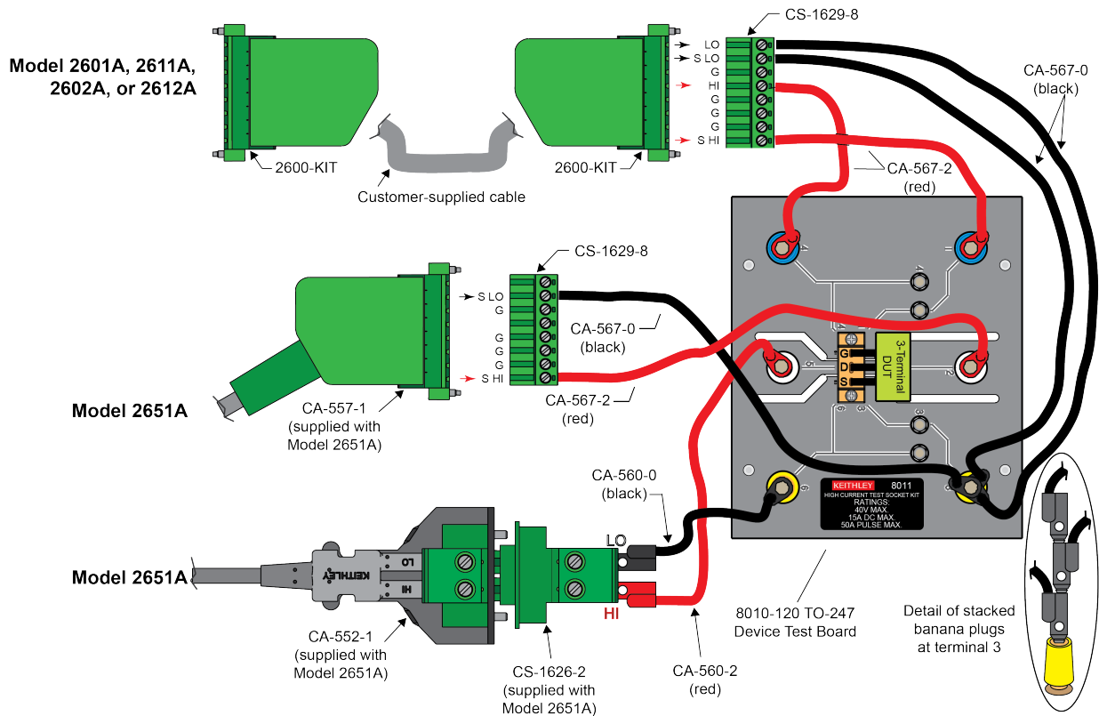
Figure 7: Connections for three-terminal device test
