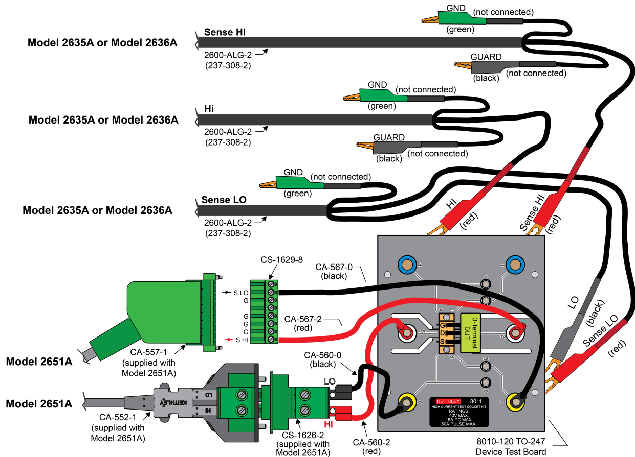
Figure 8: Connections for three-terminal device test
