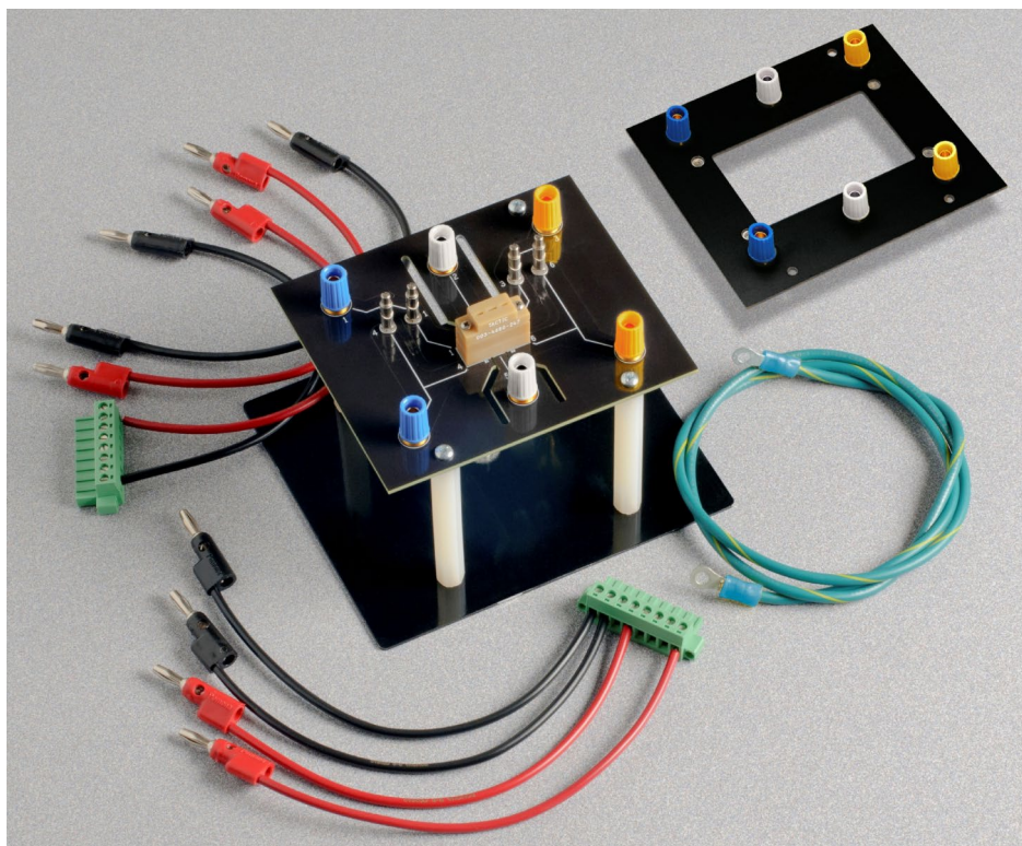
Figure 1: Model 8011 High Current Test Socket Kit*
