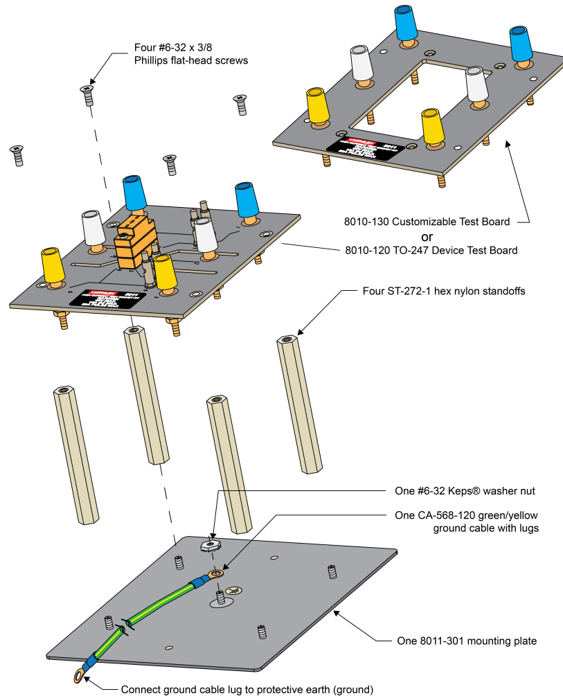
Figure 2: Model 8011 assembly
