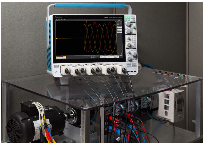
Figure 1: Voltage measurements on a three-phase motor showing the three-phase input voltages after start-up.
