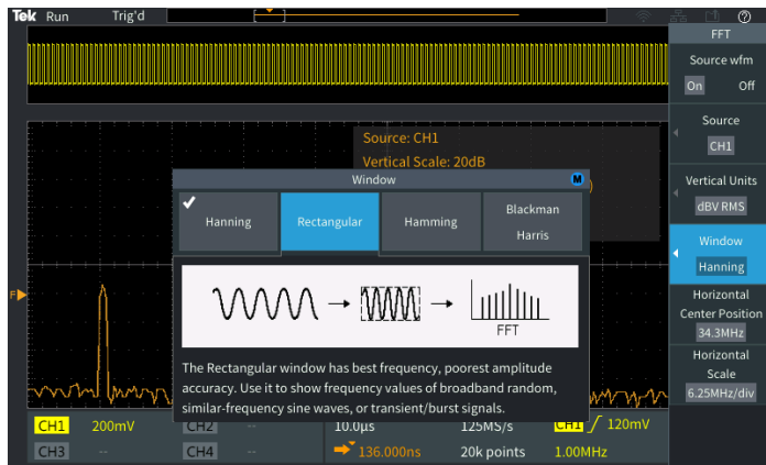
Figure 11: HelpEverywhere ® tips explain important settings.
