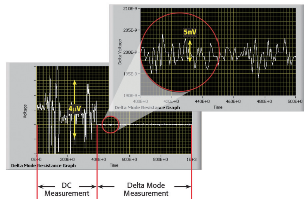
Figure 2. Results from a Model 2182A/6220 using the delta mode to measure a 10mΩ resistor
